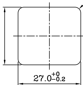
PANEL CUT-OUT
